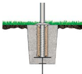
Anchor base for Patriot Series aluminum flagpole
