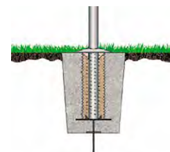
Anchor base for Patriot Series aluminum flagpole
